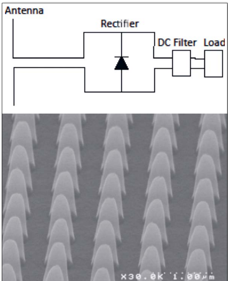
▼ FIG 3: (a) Schematic of a rectenna. (b) SEM image of nanopillar arrays obtained by nano-imprint lithography. [16]
