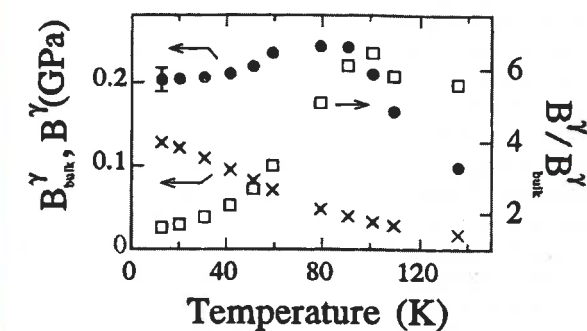
◀ Fig. 4: Tetragonal MEL stress, B^\gamma vs. temperature ( \bullet points) for the ultrathin hexagonal superlattice (\text{Ho}_6/\text{Y}_6)_{\times 100} . The difference from the bulk Ho one, B_{\text{bulk}}^\gamma ( \times points) is due to interface and non-linear MEL stresses. Also shown is the quotient B^\gamma/B_{\text{bulk}}^\gamma ( \square points) [1].
