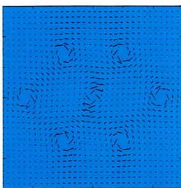
Calculated transverse optical patterns for a laser with spherical mirrors and a narrow atomic gain exciting a single family of modes show a regular "crystalline" arrangement of seven vortices. Regions of low intensity in the left-hand figure correspond to positions where the electric field phase gradient, plotted on the right, is singular. [M. Brambilla et al. , 1991].
