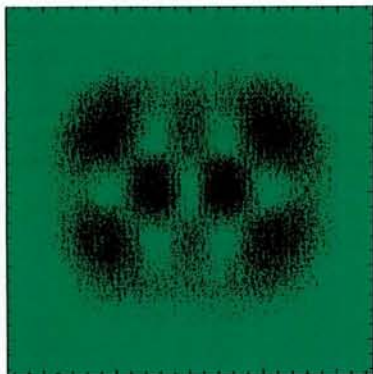
Calculated transverse optical patterns for a laser with spherical mirrors and a narrow atomic gain exciting a single family of modes show a regular "crystalline" arrangement of seven vortices. Regions of low intensity in the left-hand figure correspond to positions where the electric field phase gradient, plotted on the right, is singular. [M. Brambilla et al. , 1991].
