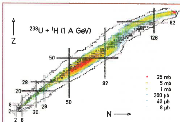
▲ Fig. 2: The 1385 identified nuclides are shown on a chart of nuclei. Numerical values are available in [9]. The magnitudes (reducing by a factor of 5) of the experimental cross-sections are indicated by a colour scale. The stable isotopes are indicated by black squares.
