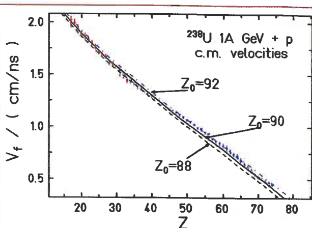
▲ Fig. 5: The mean c.m. velocity of fission fragments measured as a function of Z , the atomic number. The three lines: dashed Z_0 = 88 , full Z_0 = 90 , and dashed-dotted Z_0 = 92 , are calculated assuming Coulomb repulsion with the radius constant r_0 being fixed by taking the measured value of the velocity for symmetric fission of ^{220}\text{Th} as normalisation.
